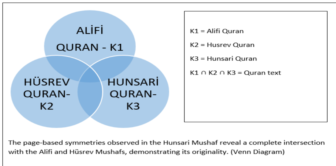
Figure 9. Venn Diagram (K1 K2 K3 Mushafs)
