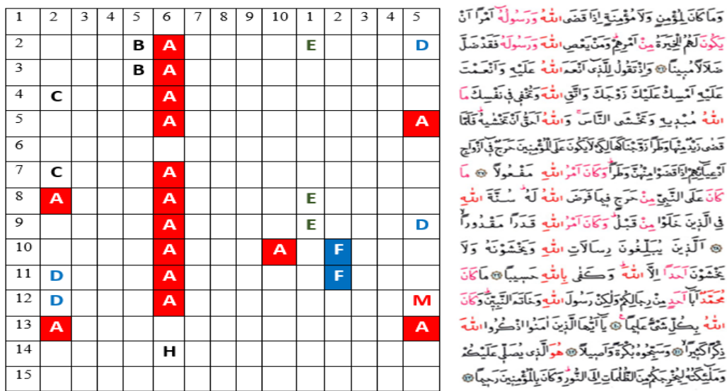
Figure 8. Husrev Mushaf Page 422 Word Coordinate Matrix
